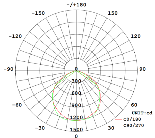
Diagram for RCM3030-04 in 3000K. Other diagrams available on request
