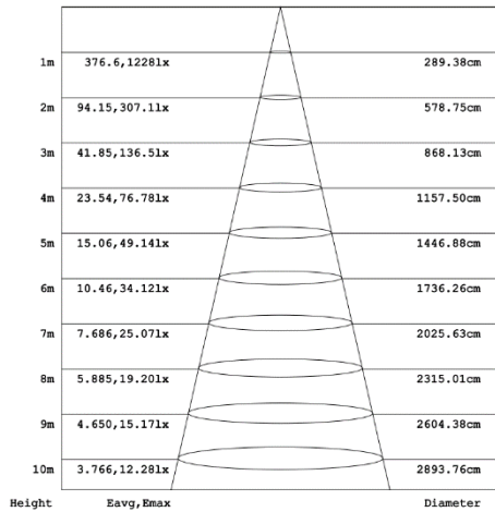
Diagram for RCM3030-04 in 3000K. Other diagrams available on request
